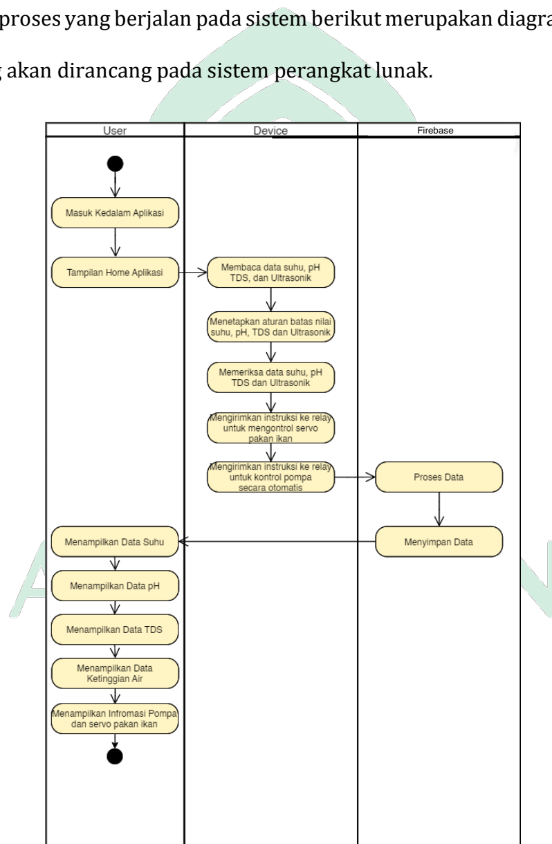
Gambar IV. 10 Activity Diagram
