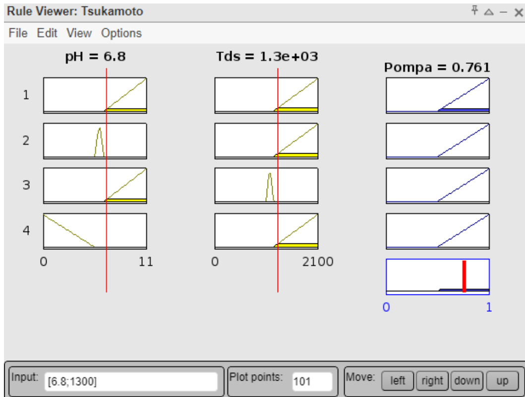
Gambar V. 11 Matlab Toolbox Fuzzy
